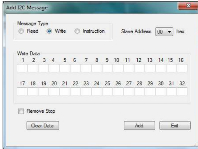
Figure 10. Add/Edit I2C Message Window - Write
