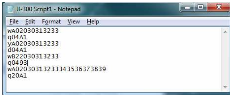
Figure 15. Script File
