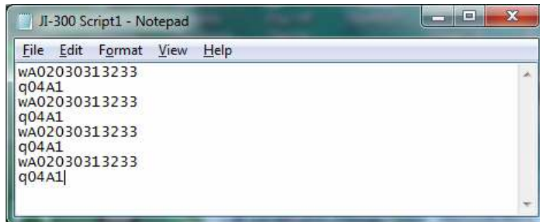
Figure 15. Script File
