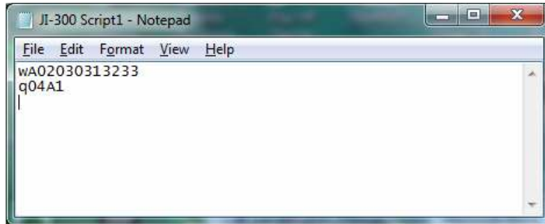
Figure 14. Script File
